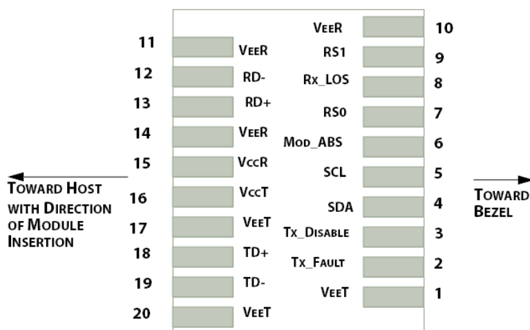
Figure1.Electrical Pin-out Details
